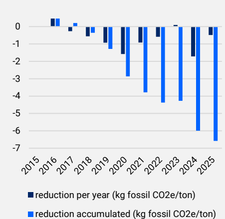
B – Reduction of Scope 1 fossil CO 2 e emissions per ton produced asphalt at all NCC Industry’s asphalt plants during 2015–2025, kg CO 2 e/ton
