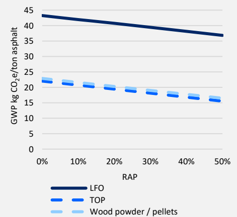
A – Effect of fuel type and amount of recycling on cradle-to-gate GWP for asphalt
